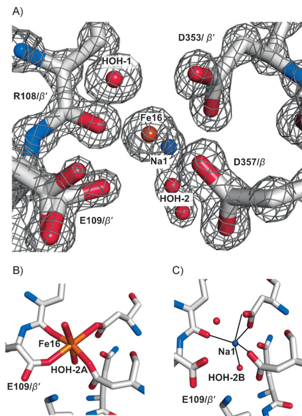
Figure 3. The refined crystallographic structure at the MMB site in the Av MoFe protein superimposed on the electron density map contoured at 2\sigma (A). The observed density of the MMB-site is interpreted as a superposition of partially occupied Fe16-bound (B) and Fe16-free (C) forms, with the latter modeled as a half-occupied \text{Na}^+ (Na1). Fe orange, O red, N blue, C gray, Na blue spheres.
